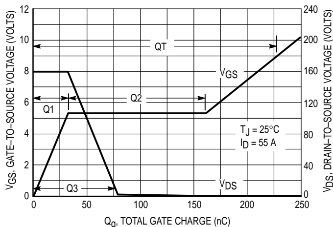
Figure 8. Gate Charge versus Gate-to-Source Voltage
