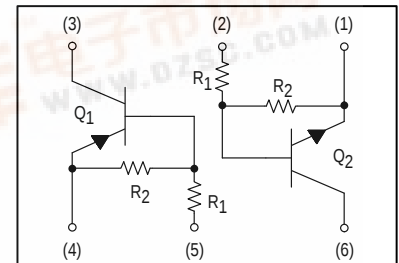
CASE 419B-01, STYLE 1 SOT-363
