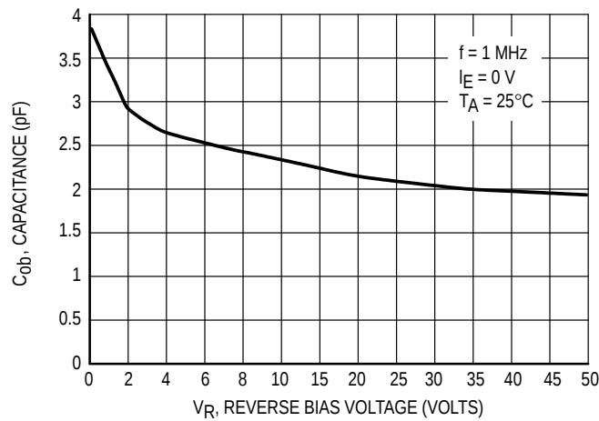
Figure 34. Output Capacitance
