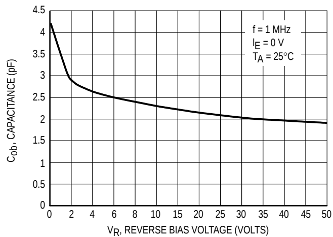
Figure 39. Output Capacitance
