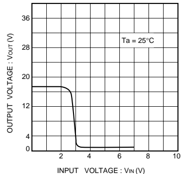
Fig.4 I / O characteristics
