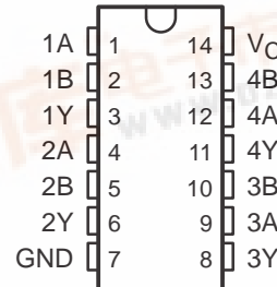
SN54ACT32 ... J OR W PACKAGE SN74ACT32 ... D, DB, N, OR PW PACKAGE (TOP VIEW)
