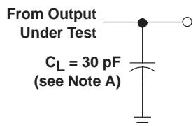
LOAD CIRCUIT FOR t r AND t f
