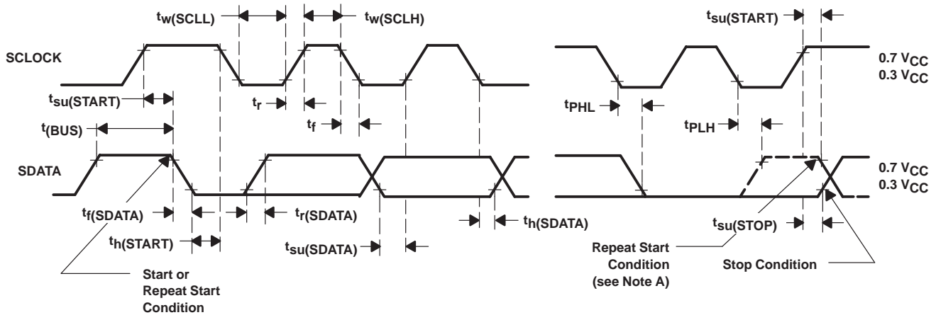
VOLTAGE WAVEFORMS
