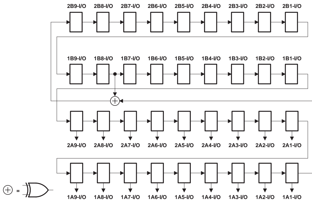
Figure 7. 36-Bit PRPG Configuration ( 1OEAB = 2OEAB = 0 , \overline{1OEBA} = \overline{2OEBA} = 0 )
