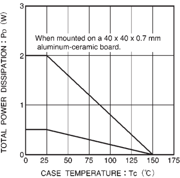
Fig.1 Total power dissipation vs. case temperature
