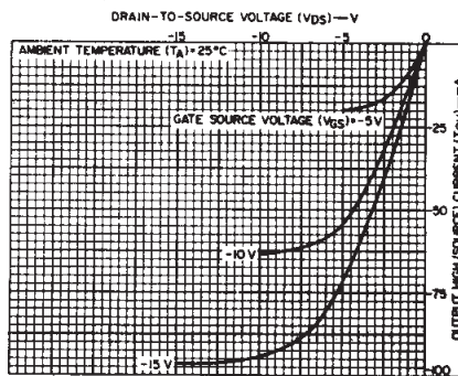
Fig. 5 - Minimum output high (source) characteristics.
