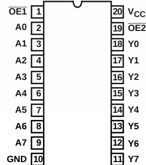
CD54HC541, CD54HCT541 (CERDIP) CD74HC541, CD74HCT541 (PDIP, SOIC) TOP VIEW
