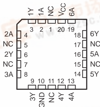
SN54HCT04 ... FK PACKAGE (TOP VIEW)
