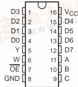
SN54HC251 ... J OR W PACKAGE SN74HC251 ... D, DB, OR N PACKAGE (TOP VIEW)
