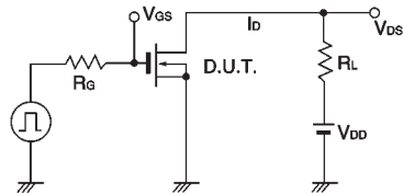
● Switching characteristics measurement circuit
