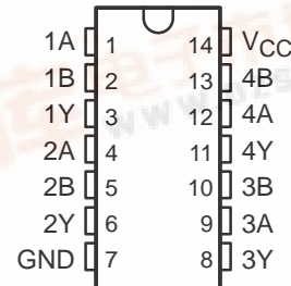
SN54AHC32 . . . J OR W PACKAGE SN74AHC32 . . . D, DB, DGV, N, OR PW PACKAGE (TOP VIEW)
