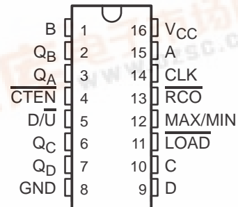
SN54ALS191 ... J PACKAGE SN74ALS191A ... D OR N PACKAGE (TOP VIEW)
