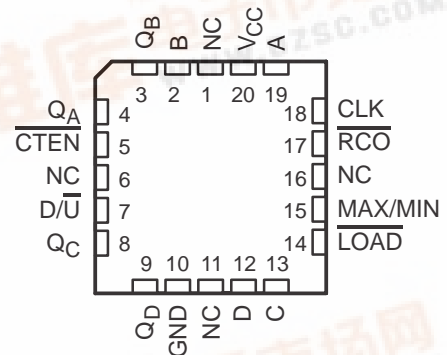
SN54ALS191 ... FK PACKAGE (TOP VIEW)
