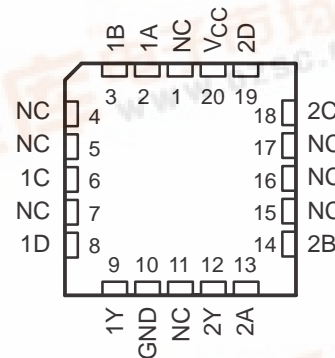
SN54F21 ... FK PACKAGE (TOP VIEW)
