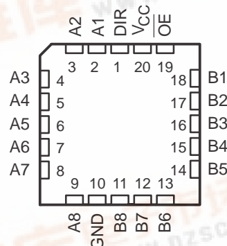
SN54F245 . . . FK PACKAGE (TOP VIEW)
