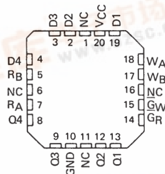
SN54LS670 . . . FK PACKAGE
