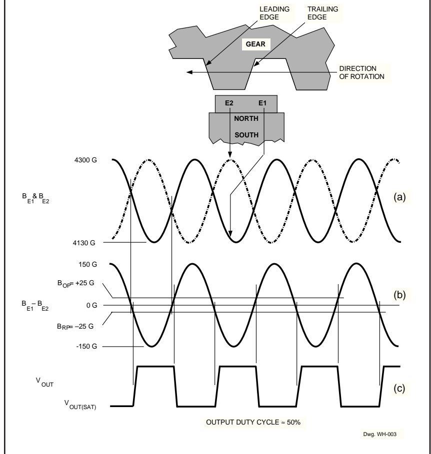
Figure 3 GEAR-TOOTH SENSOR OPERATION
