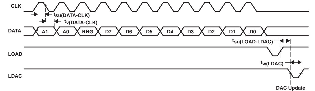
Figure 2. LDAC-Controlled Update
