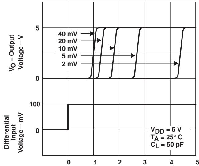
LOW-TO-HIGH-LEVEL OUTPUT RESPONSE FOR VARIOUS INPUT OVERDRIVES
