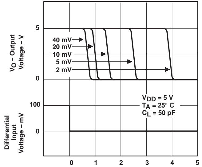
HIGH-TO-LOW-LEVEL OUTPUT RESPONSE FOR VARIOUS INPUT OVERDRIVES
