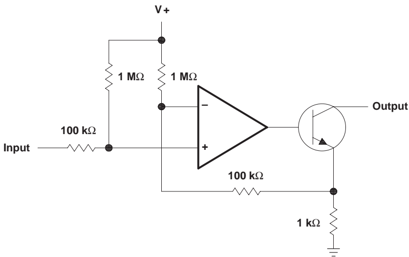
Figure 13. Voltage-Controlled Current Source
