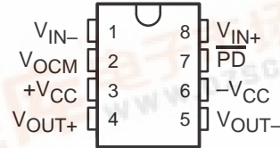
THS4151 D OR DGN PACKAGE (TOP VIEW)
