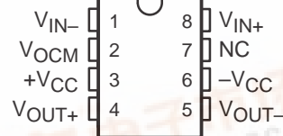
THS4151 D OR DGN PACKAGE (TOP VIEW)
