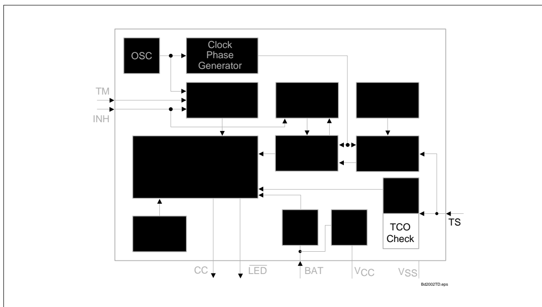
Figure 4. Block Diagram
