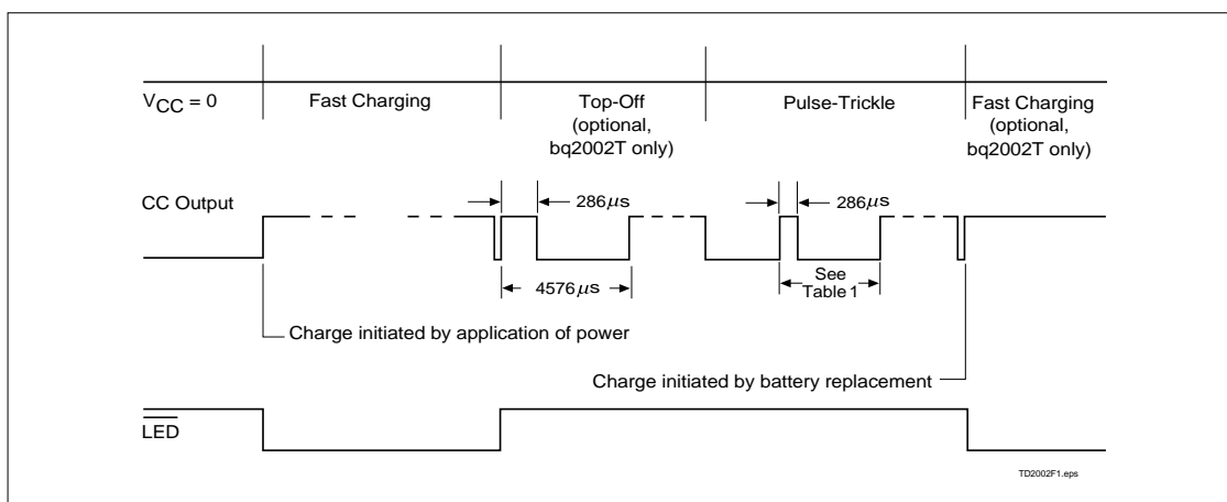
Figure 5. Charge Cycle Phases
