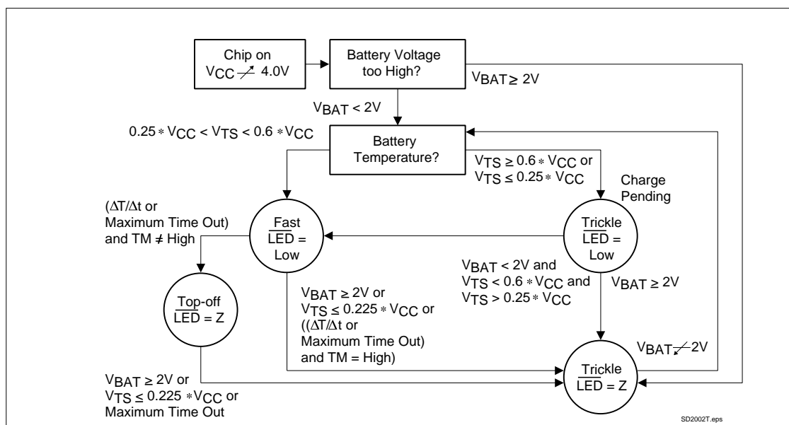
Figure 3. bq2002T State Diagram
