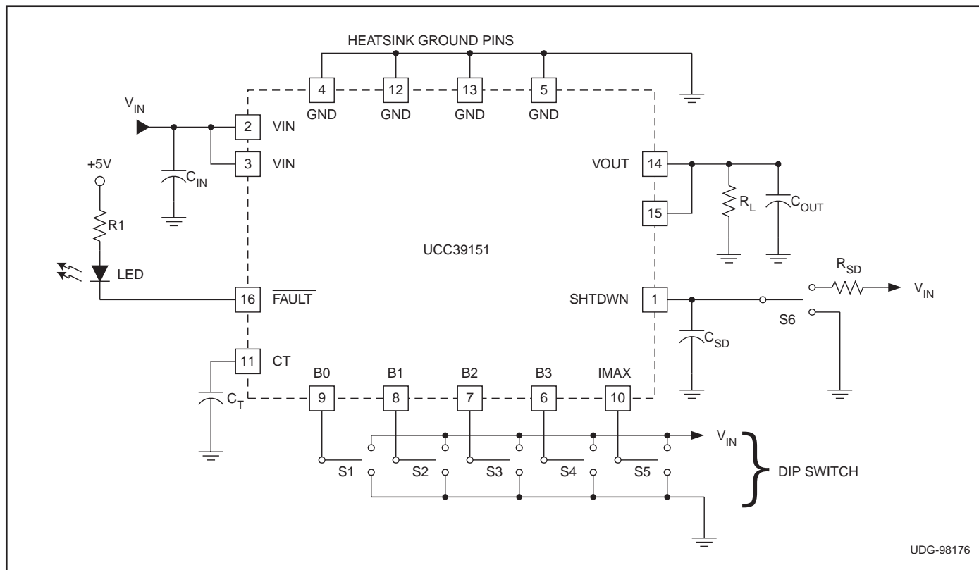
Figure 1. Evaluation circuit.
