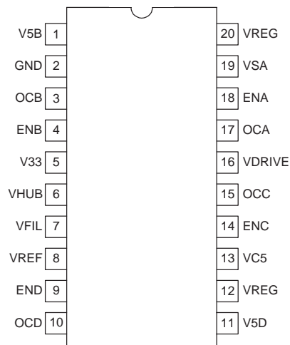
DIP-20 (Top View) N Package
