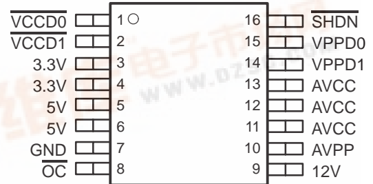
DB PACKAGE (TOP VIEW)
