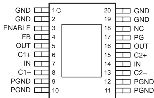
PWP PACKAGE (TPS60121, TPS60123, TPS60125) (TOP VIEW)
