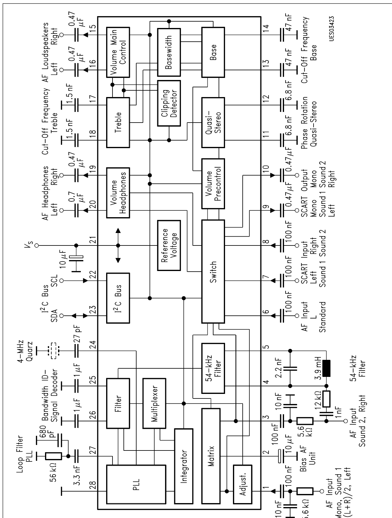
Application Circuit 3
