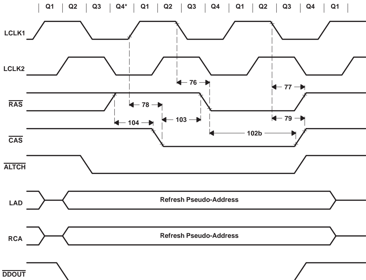
Figure 43. \overline{\text{CAS}} -Before- \overline{\text{RAS}} Refresh: \overline{\text{RAS}} and \overline{\text{CAS0}}-\overline{\text{CAS3}}
