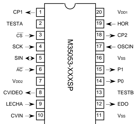
Outline 20P4B
