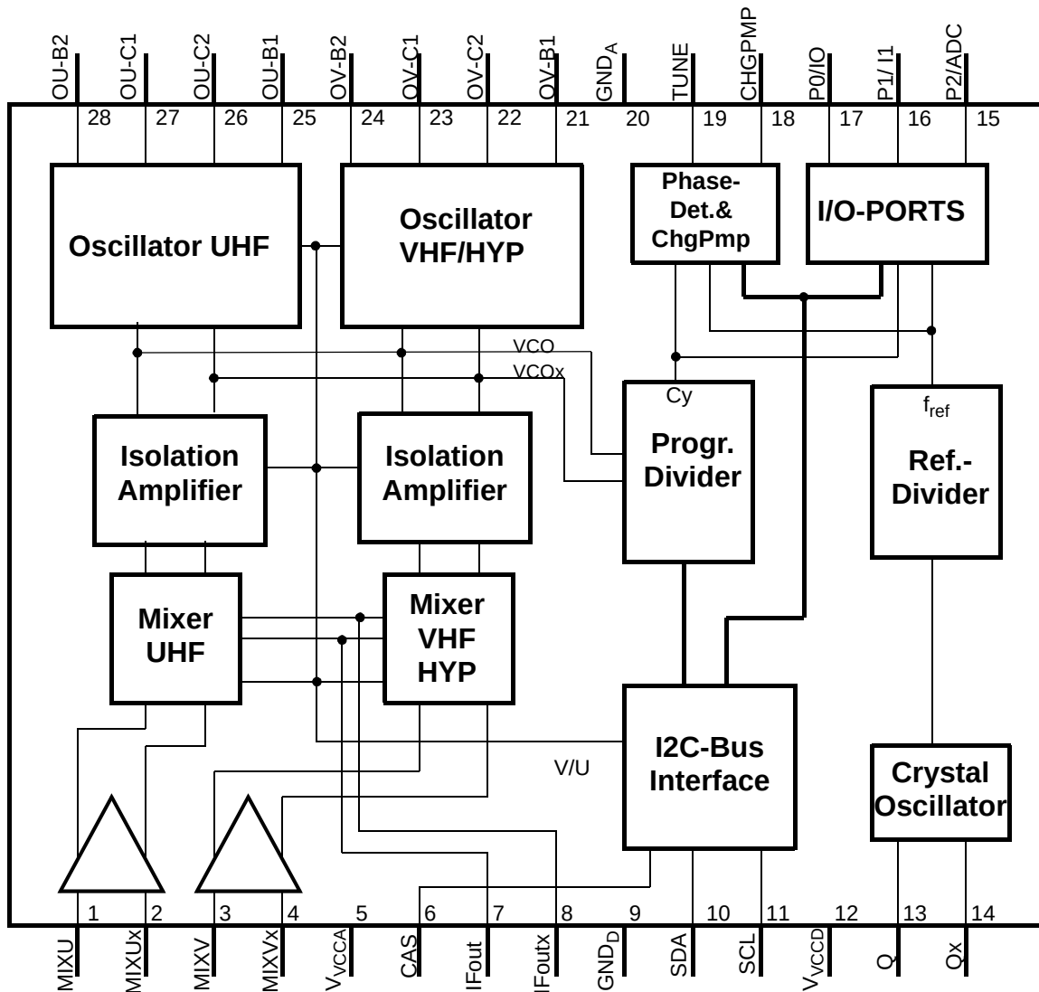
Figure 3-2 Block Diagram
