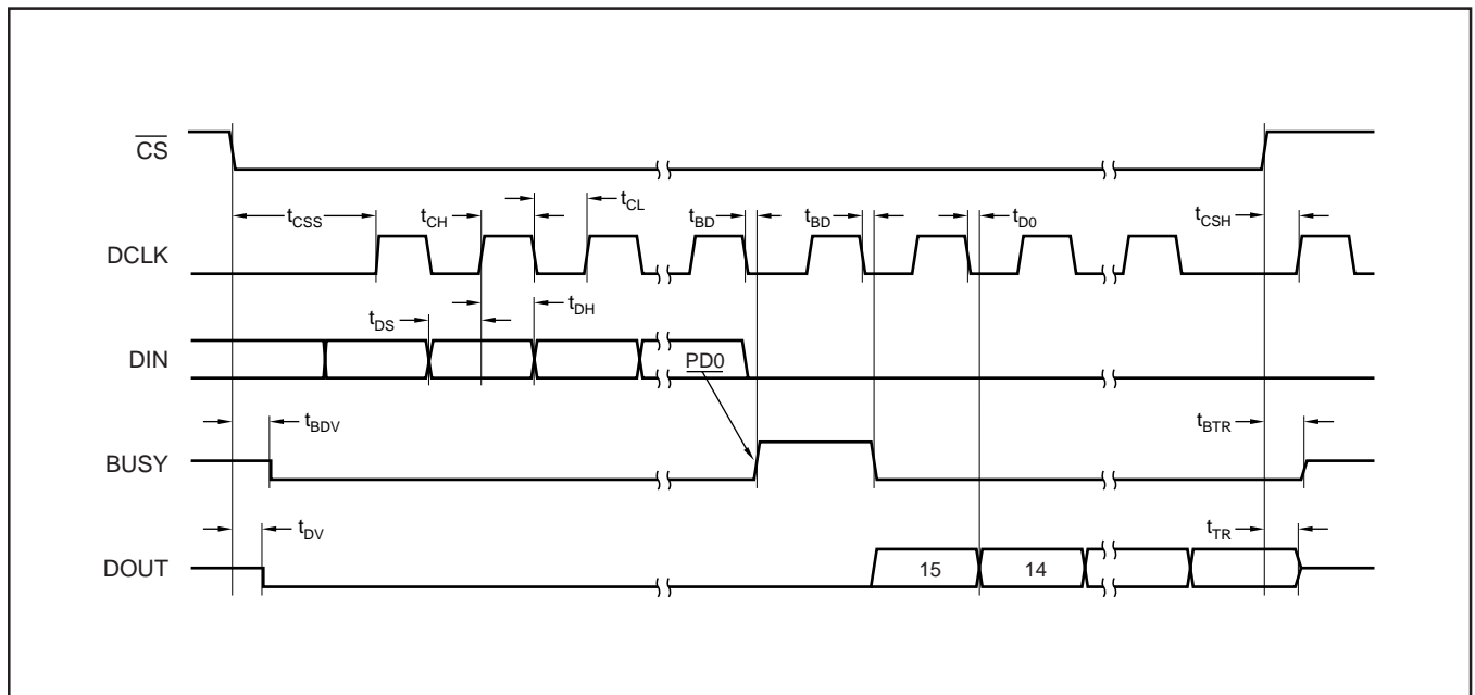
FIGURE 4. Detailed Timing Diagram.
