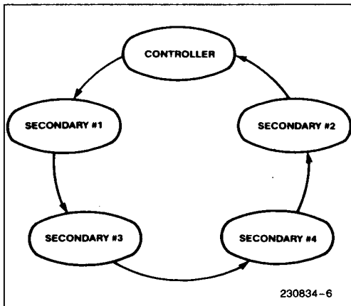
Figure 6. An SDLC Loop
