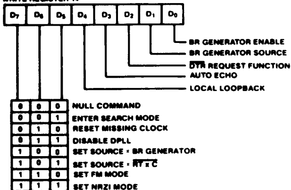
Figure 10. Write Register Bit Functions (Continued)
