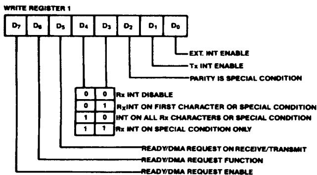
Figure 10. Write Register Bit Functions
