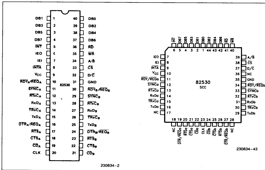
Figure 2. Pin Configurations
