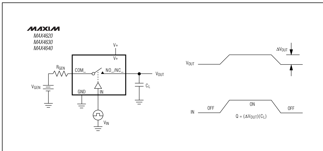
Figure 4. Charge Injection
