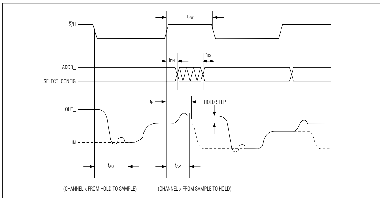
Figure 2. Timing Diagram
