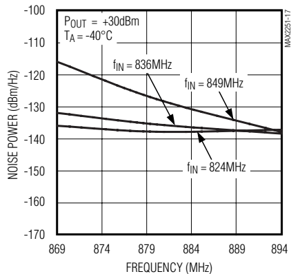
NOISE POWER vs. FREQUENCY
