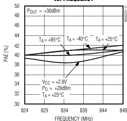
POWER-ADDED EFFICIENCY vs. FREQUENCY
