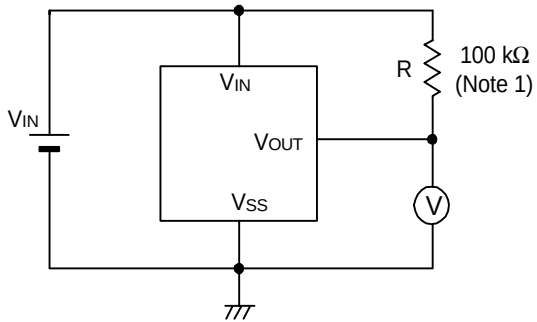
Circuit 1
