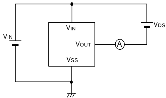
Circuit 4
