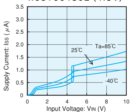
XC61CC4502 (4.5 V)
