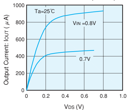
XC61CC3602 (3.6V)
