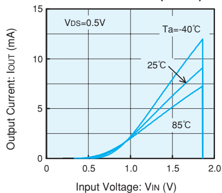
XC61CC1802 (1.8V)
