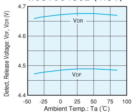
XC61CC4502 (4.5 V)
