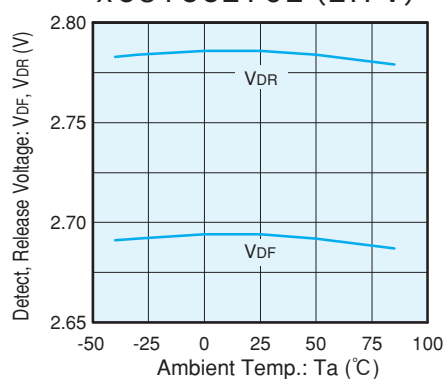
XC61CC2702 (2.7 V)
