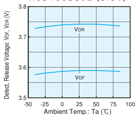
XC61CC3602 (3.6 V)
