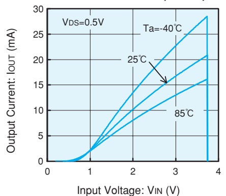
XC61CC3602 (3.6V)
