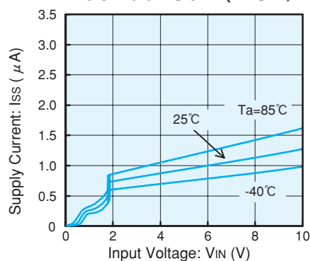
XC61CC1802 (1.8 V)
