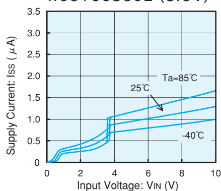
XC61CC3602 (3.6 V)
