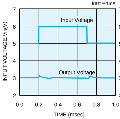
XC62HR3002 (3V)
