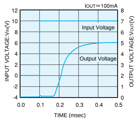
XC62HR5002 (5V)
