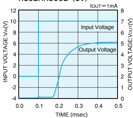
XC62HR5002 (5V)
