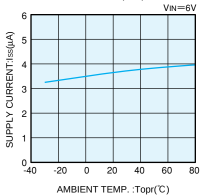
XC62HR5002 (5V)
