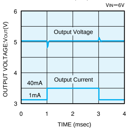
XC62HR5002 (5V)
