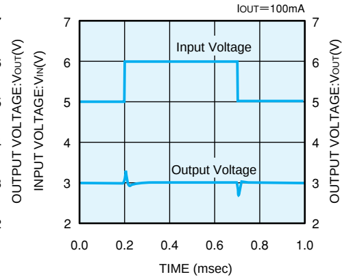
XC62HR3002 (3V)
