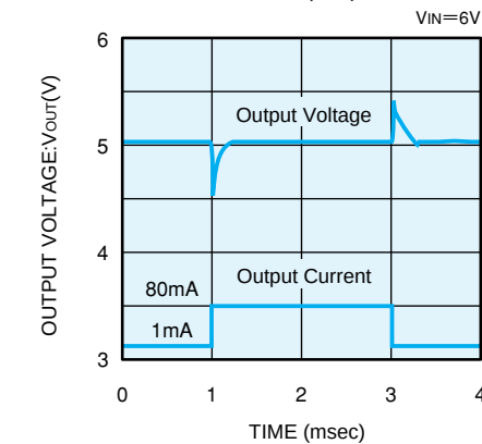
XC62HR5002 (5V)
