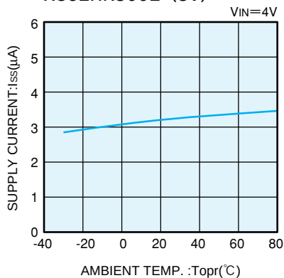
XC62HR3002 (3V)
