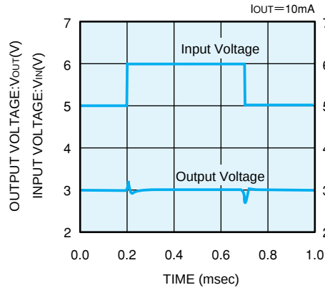
XC62HR3002 (3V)
