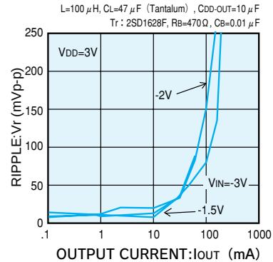
RIPPLE vs. OUTPUT CURRENT
