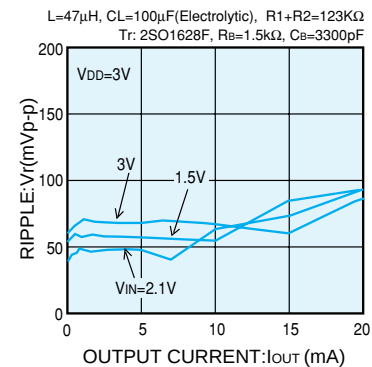
RIPPLE vs. OUTPUT CURRENT
