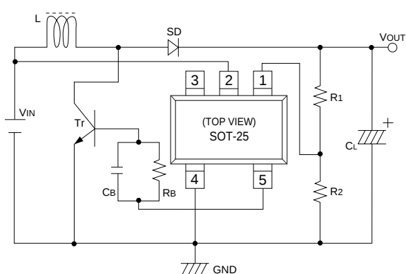
Fig.8 XC6383F Application
