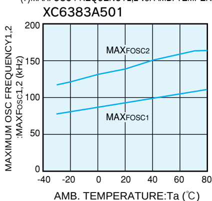
(7) MAX. OSC FREQUENCY 1,2 vs. AMB. TEMPERATURE
