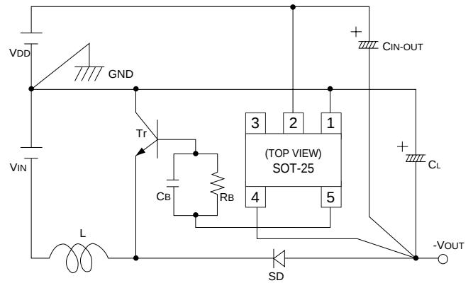
Fig.10 XC6383F Application
