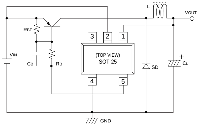
Fig.7 XC6383E Application
