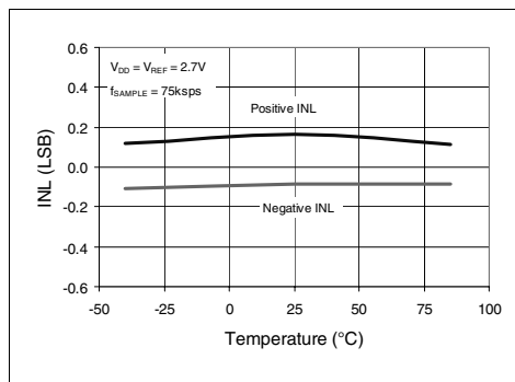
FIGURE 2-10: Integral Nonlinearity (INL) vs. Temperature ( V_{DD} = 2.7V ).
