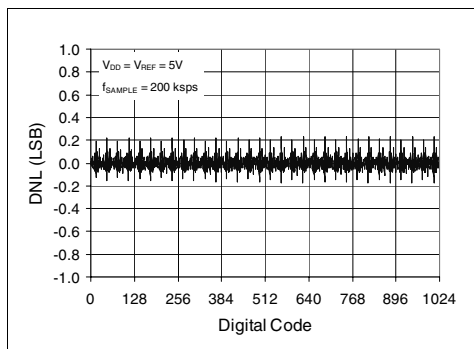
FIGURE 2-13: Differential Nonlinearity (DNL) vs. Code (Representative Part).
