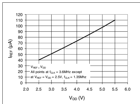
FIGURE 2-34: I_{REF} vs. V_{DD} .
