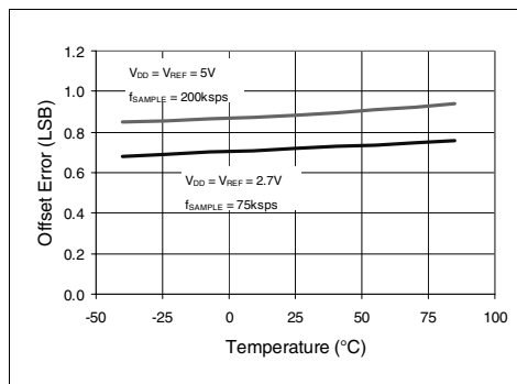
FIGURE 2-22: Offset Error vs. Temperature.
