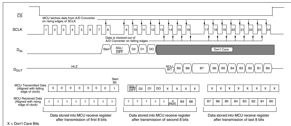
FIGURE 6-1: SPI Communication with the MCP3004/3008 using 8-bit segments (Mode 0,0: SCLK idles low).
