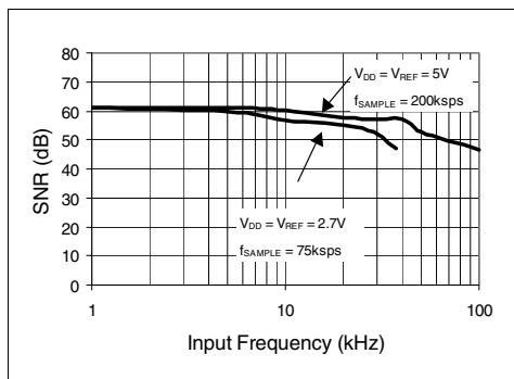
FIGURE 2-20: Signal to Noise (SNR) vs. Input Frequency.
