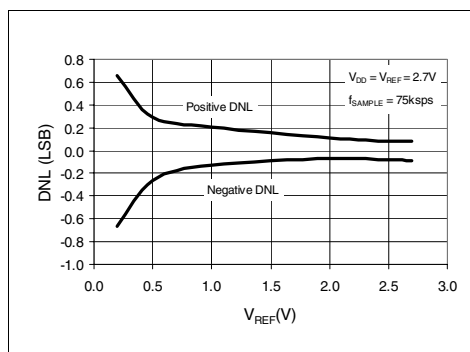
FIGURE 2-12: Differential Nonlinearity (DNL) vs. V_{REF} ( V_{DD} = 2.7V ).
