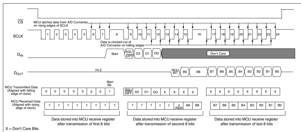
FIGURE 6-2: SPI Communication with the MCP3004/3008 using 8-bit segments (Mode 1,1: SCLK idles high).
