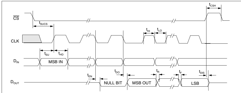
FIGURE 1-1: Serial Interface Timing.
