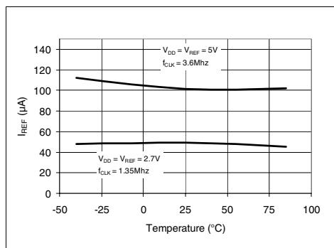
FIGURE 2-36: I_{REF} vs. Temperature.
