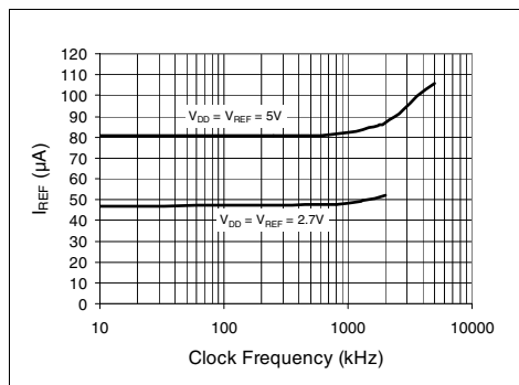
FIGURE 2-35: I_{REF} vs. Clock Frequency.
