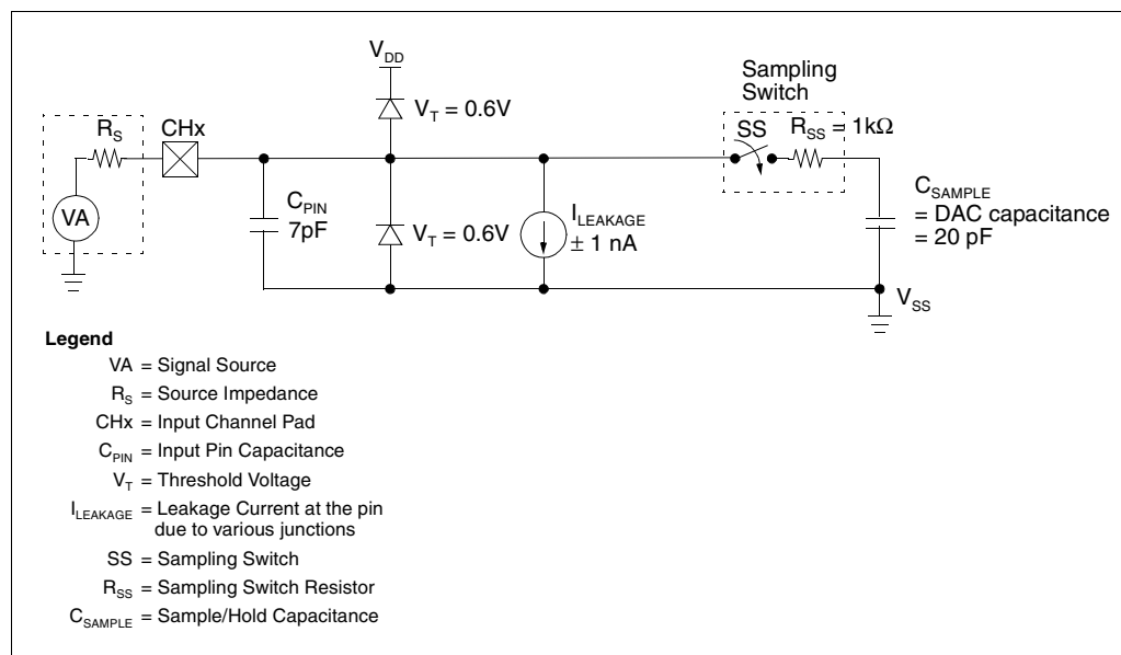
FIGURE 4-1: Analog Input Model
