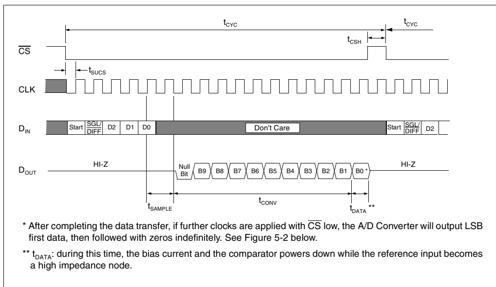
FIGURE 5-1: Communication with the MCP3204 or MCP3208.
