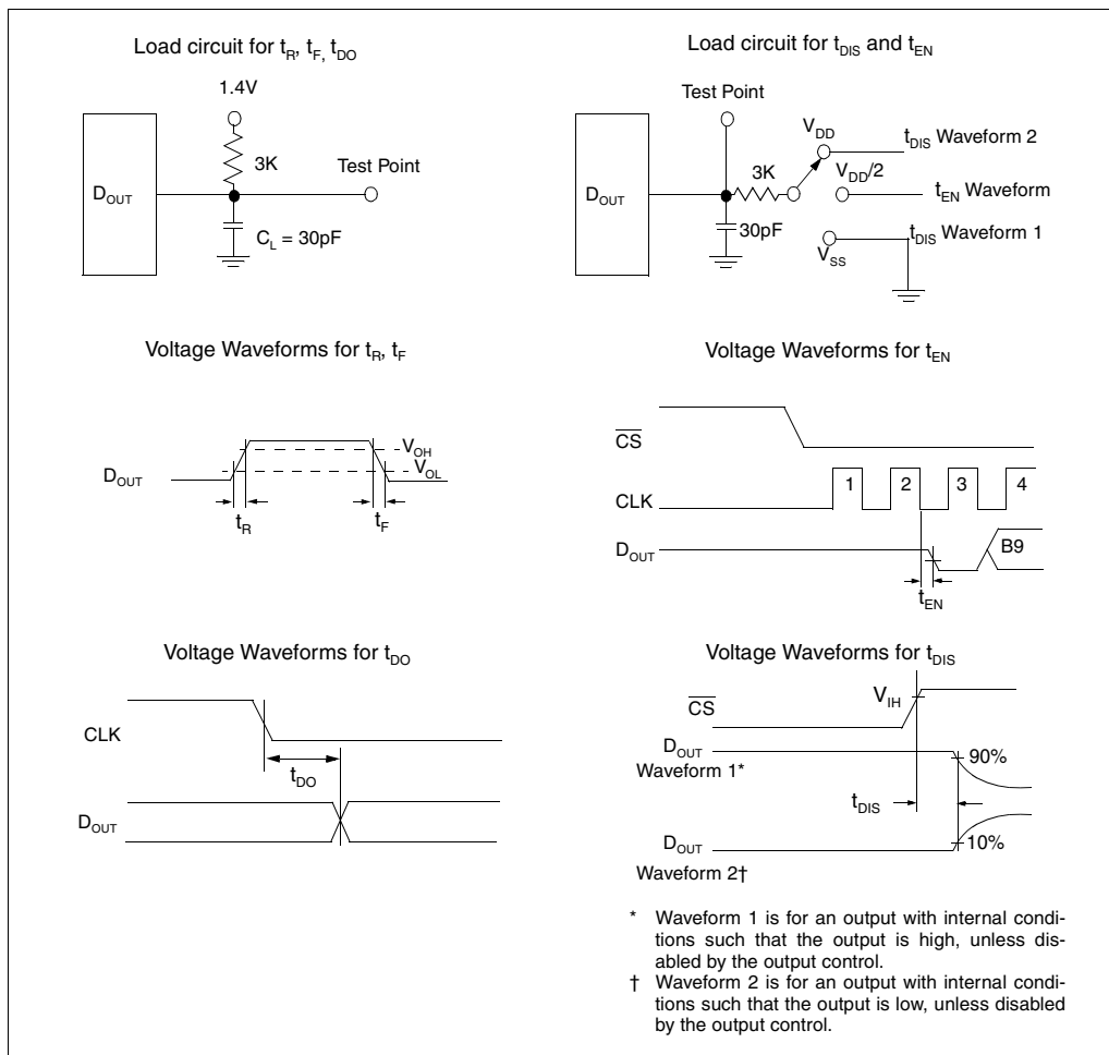
FIGURE 1-2: Test Circuits.
