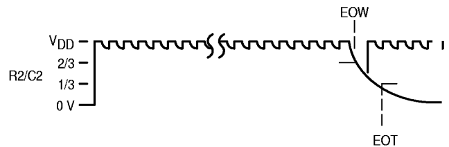
Figure 16. R-C Decay on Pin 10 (R2/C2)
