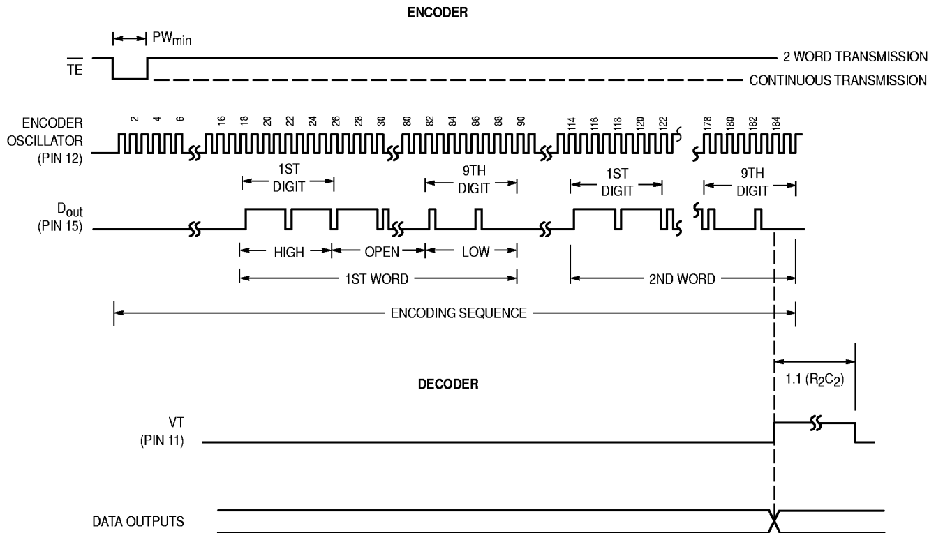
Figure 10. Timing Diagram
