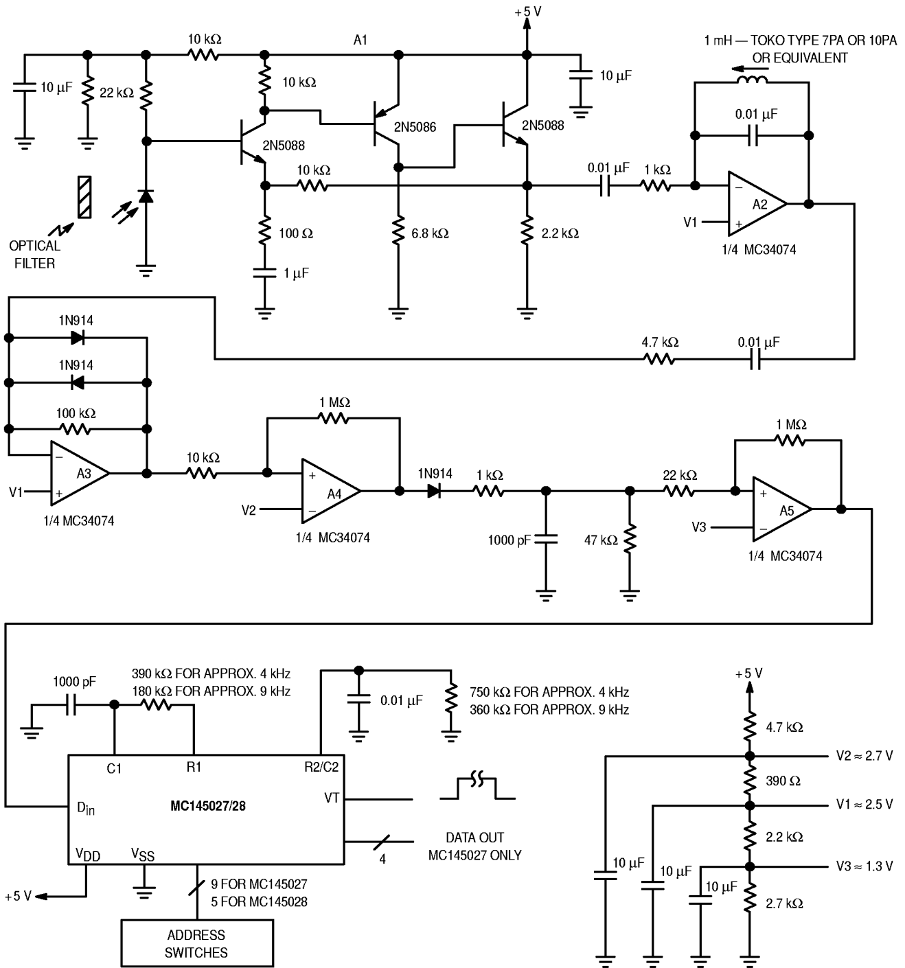
Figure 20. Infrared Receiver
