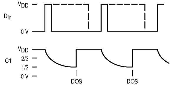
Figure 15. R-C Decay on Pin 7 (C1)
