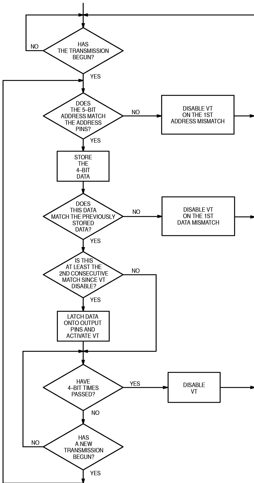
Figure 13. MC145027 Flowchart
