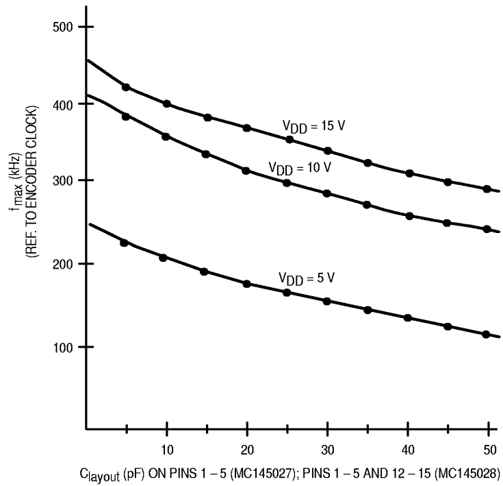
Figure 12. f_{max} vs C_{layout} — Decoders Only
