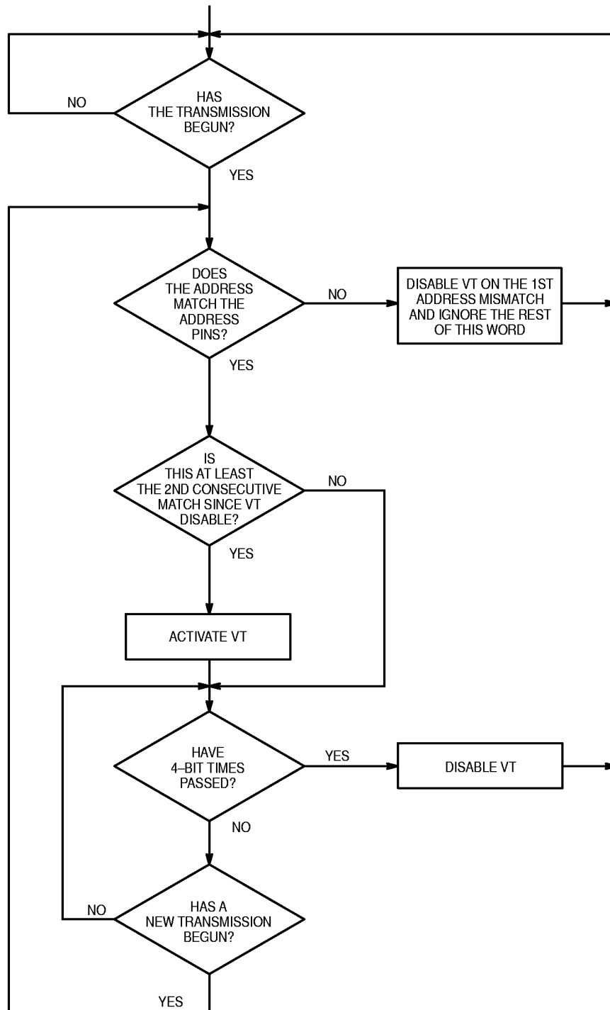
Figure 14. MC145028 Flowchart
