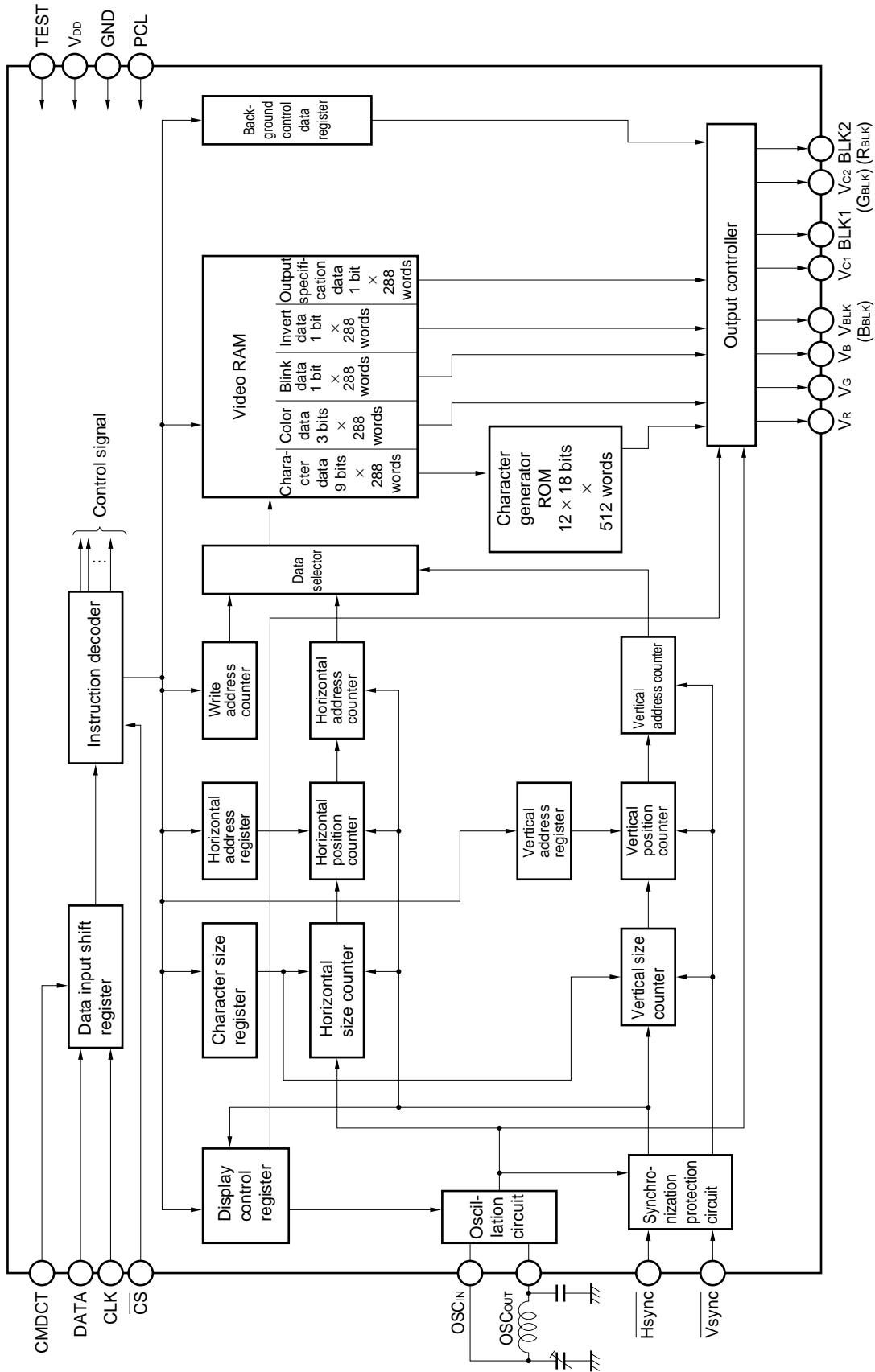
Figure 1-7. \mu PD6466 Block Diagram
