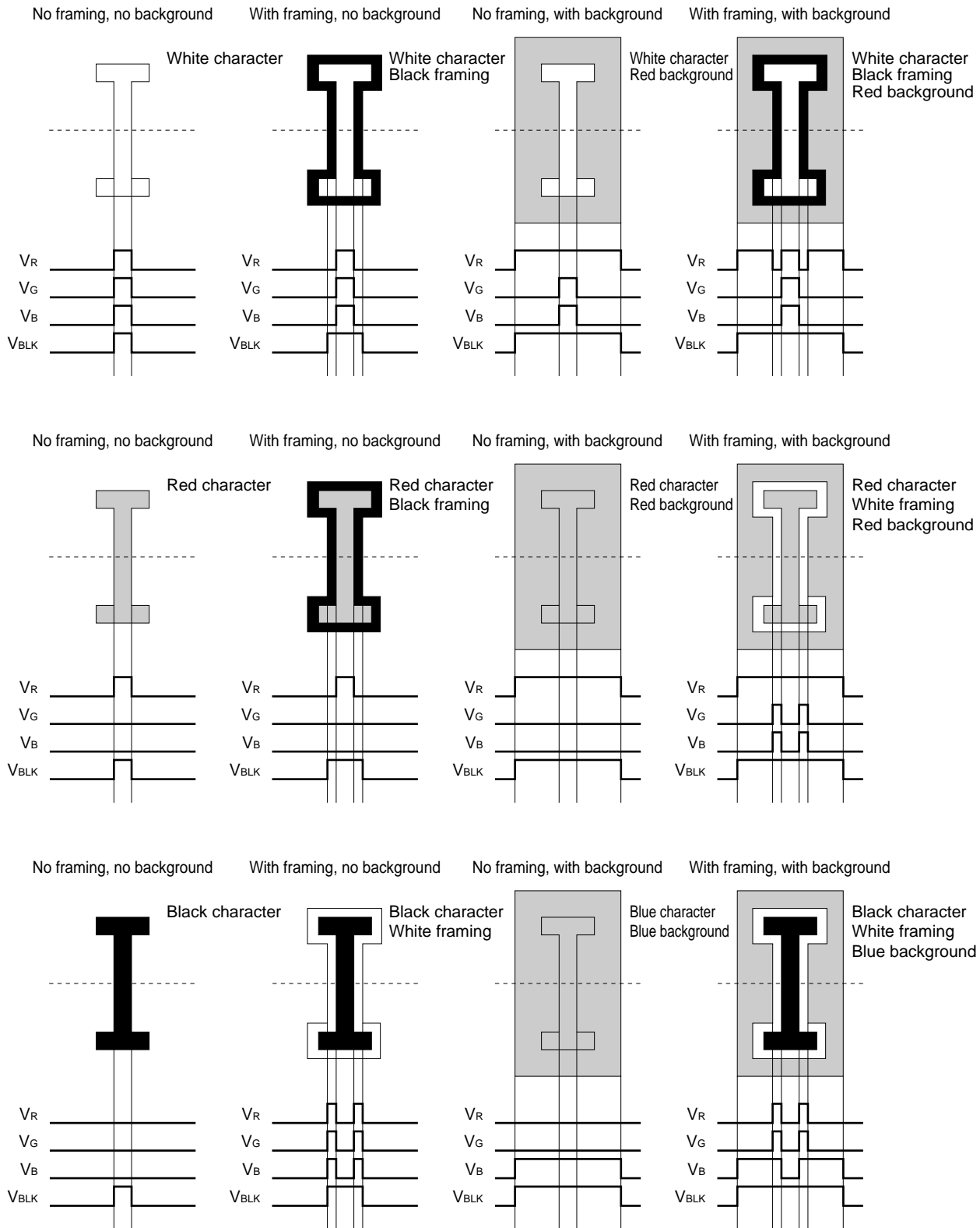
Figure 2-17. Output Pins: Sample R, G, B, and BLK Output Images When RGB + Vc1 + Vc2 Is Selected
