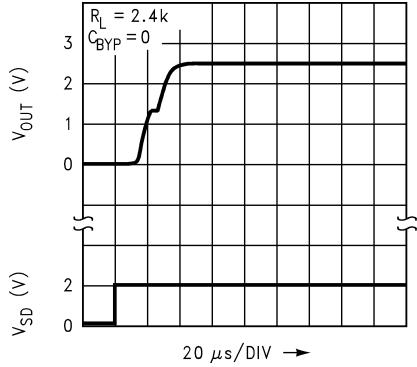
Turn-ON Waveform
