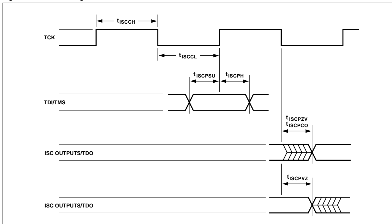
Figure 43. ISC Timing
