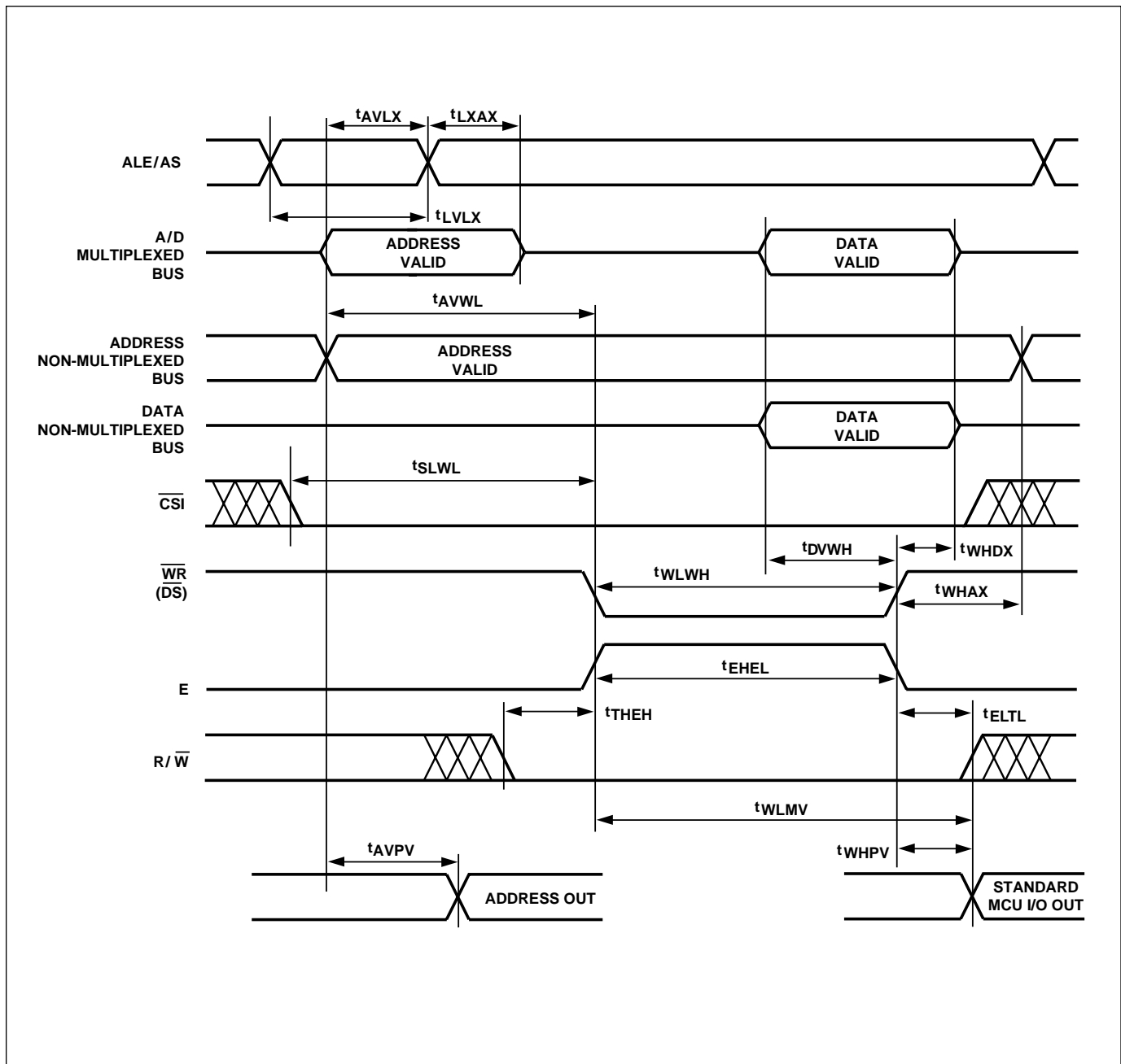
Figure 34. Write Timing
