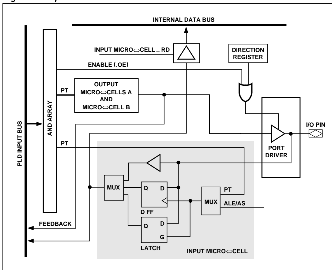
Figure 13. Input Micro⇌Cell
