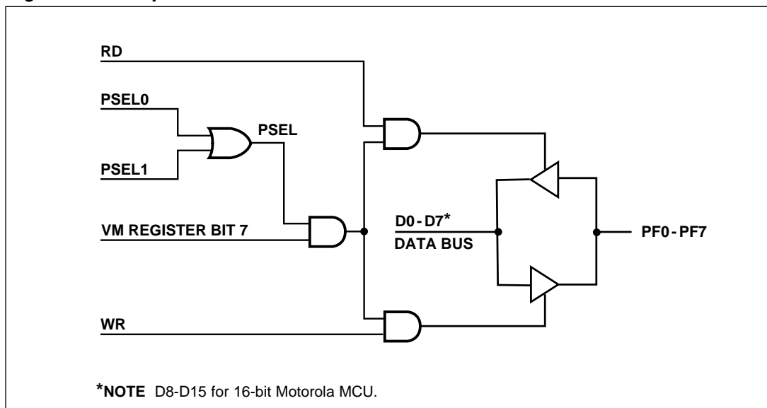
Figure 25. Peripheral I/O Mode
