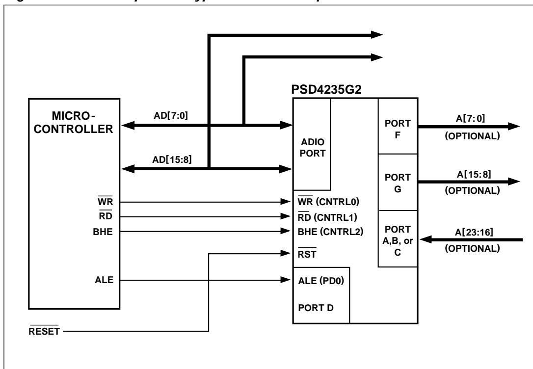
Figure 16. An Example of a Typical 16-Bit Multiplexed Bus Interface
