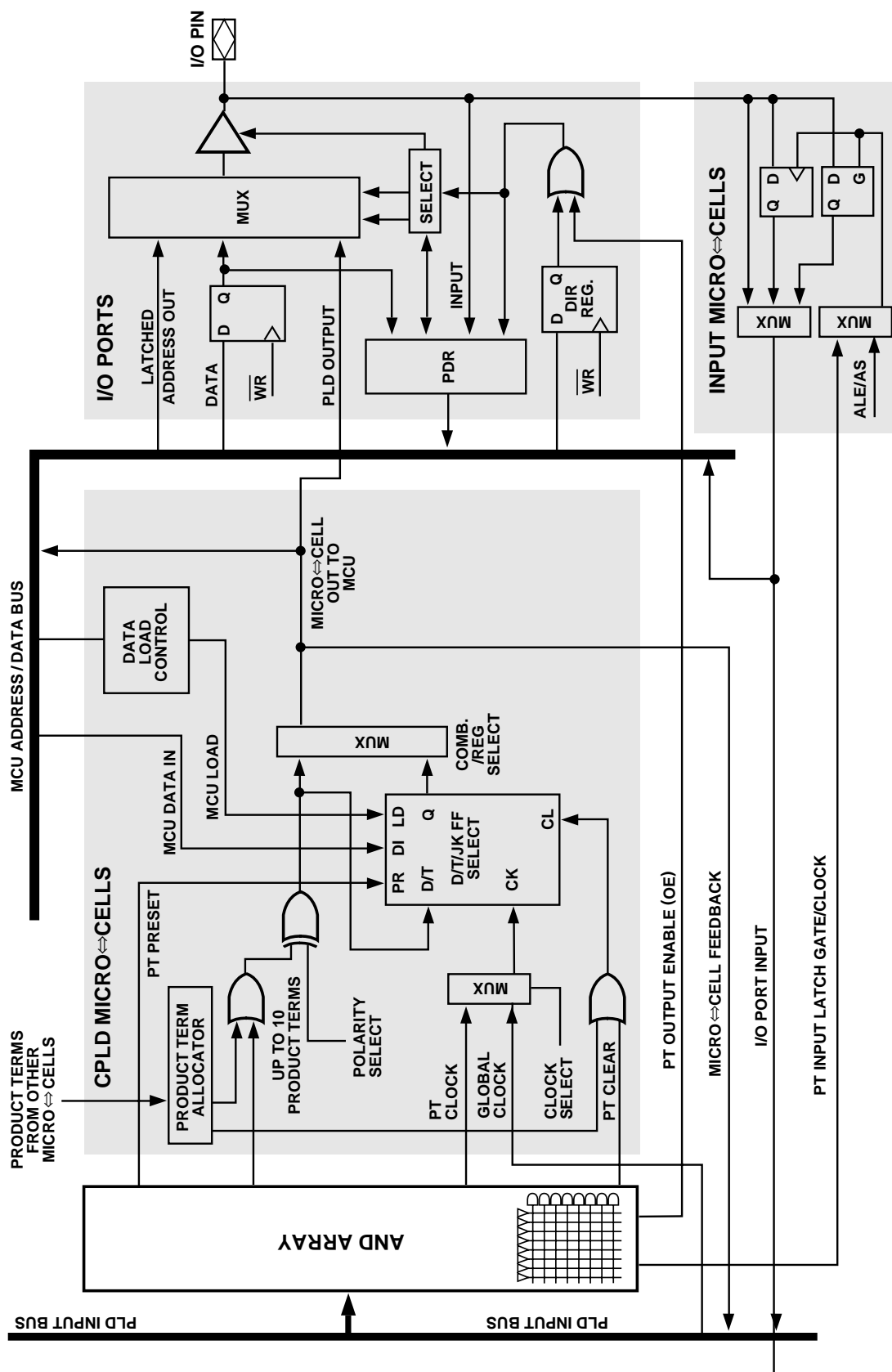
Figure 11. The Micro \leftrightarrow Cell and I/O Port
