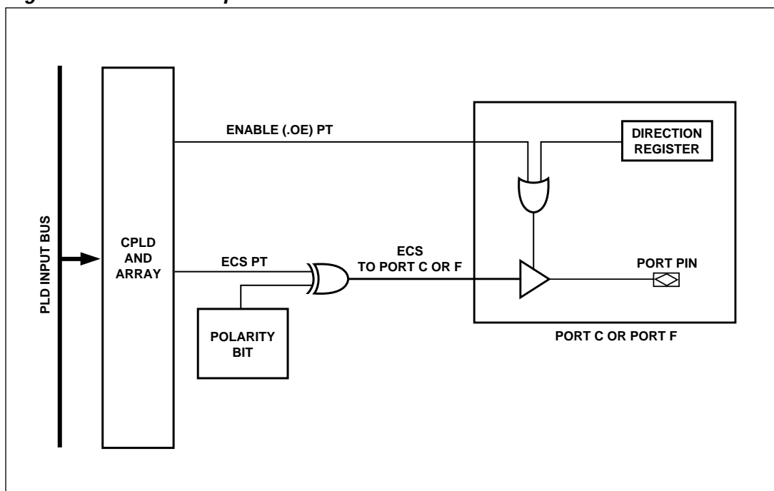
Figure 15. External Chip Select
