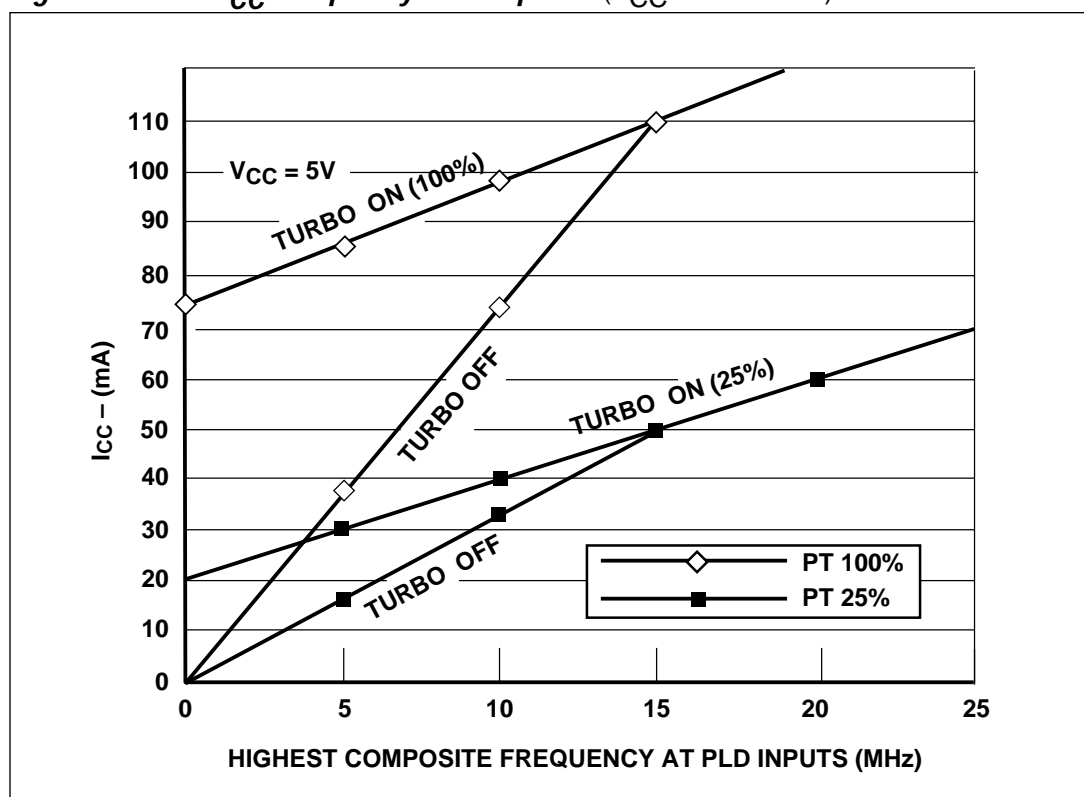
Figure 32. PLD I_{CC} /Frequency Consumption ( V_{CC} = 5\text{ V} \pm 10\% )
