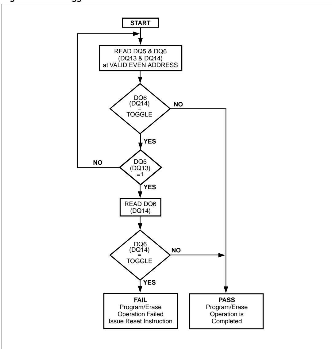
Figure 4. Data Toggle Flow Chart
