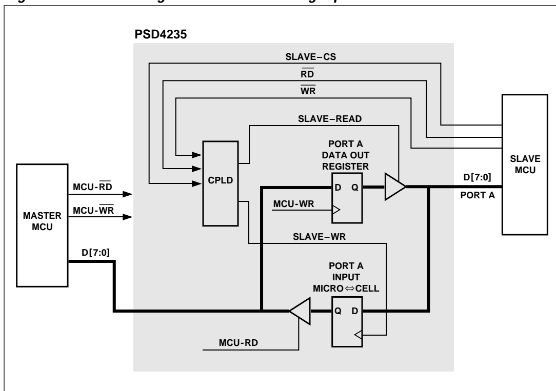
Figure 14. Handshaking Communication Using Input Micro \leftrightarrow Cells
