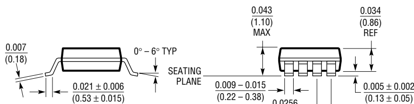
MS8 Package 8-Lead Plastic MSOP (LTC DWG # 05-08-1660)
