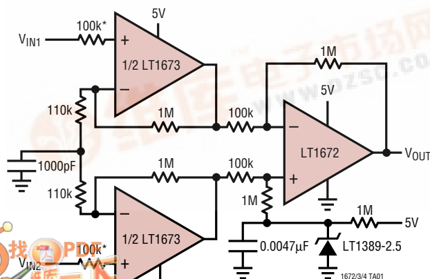
Single Supply, 60 \mu W Precision Instrumentation Amplifier
