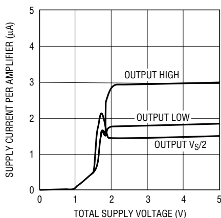
Figure 1. Start-Up Characteristics
