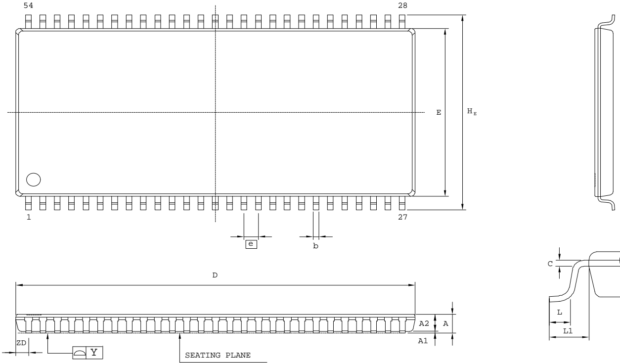
Controlling Dimension : Millimeters
