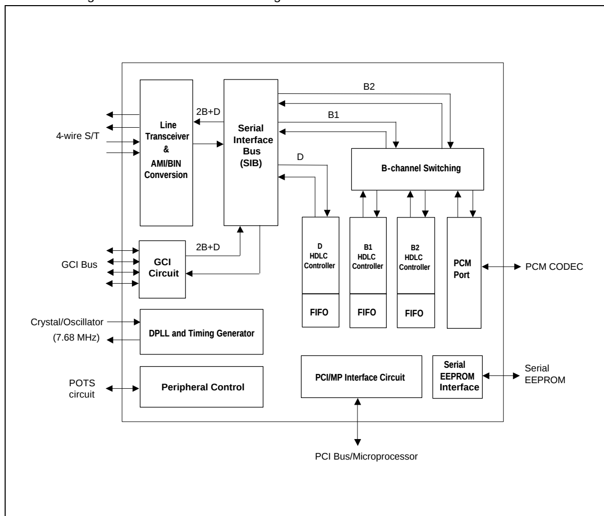
Fig.6.1 W6692A Functional Block Diagram
