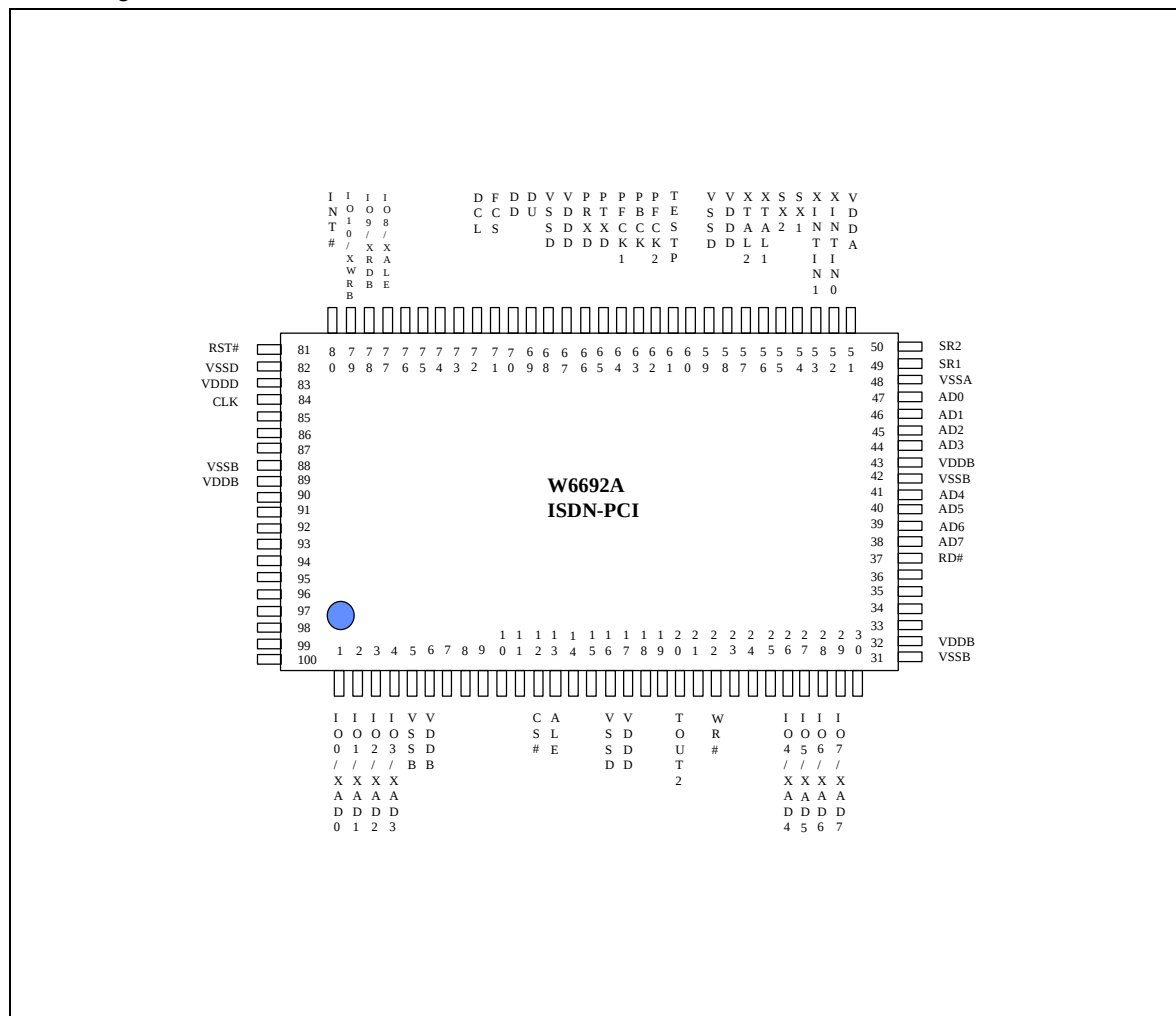
Fig.3.2 W6692A Pin Configuration - Intel Bus Mode
