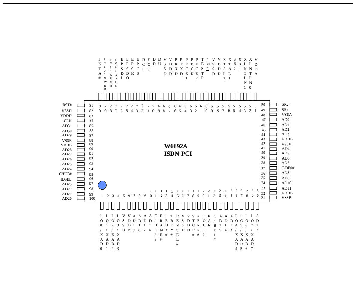
Fig.3.1 W6692A Pin Configuration-pci Mode
