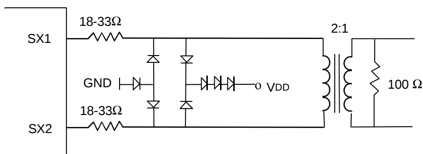
Fig.7.3 External Transmitter Circuitry
