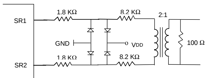
Fig.7.4 External Receiver Circuitry
