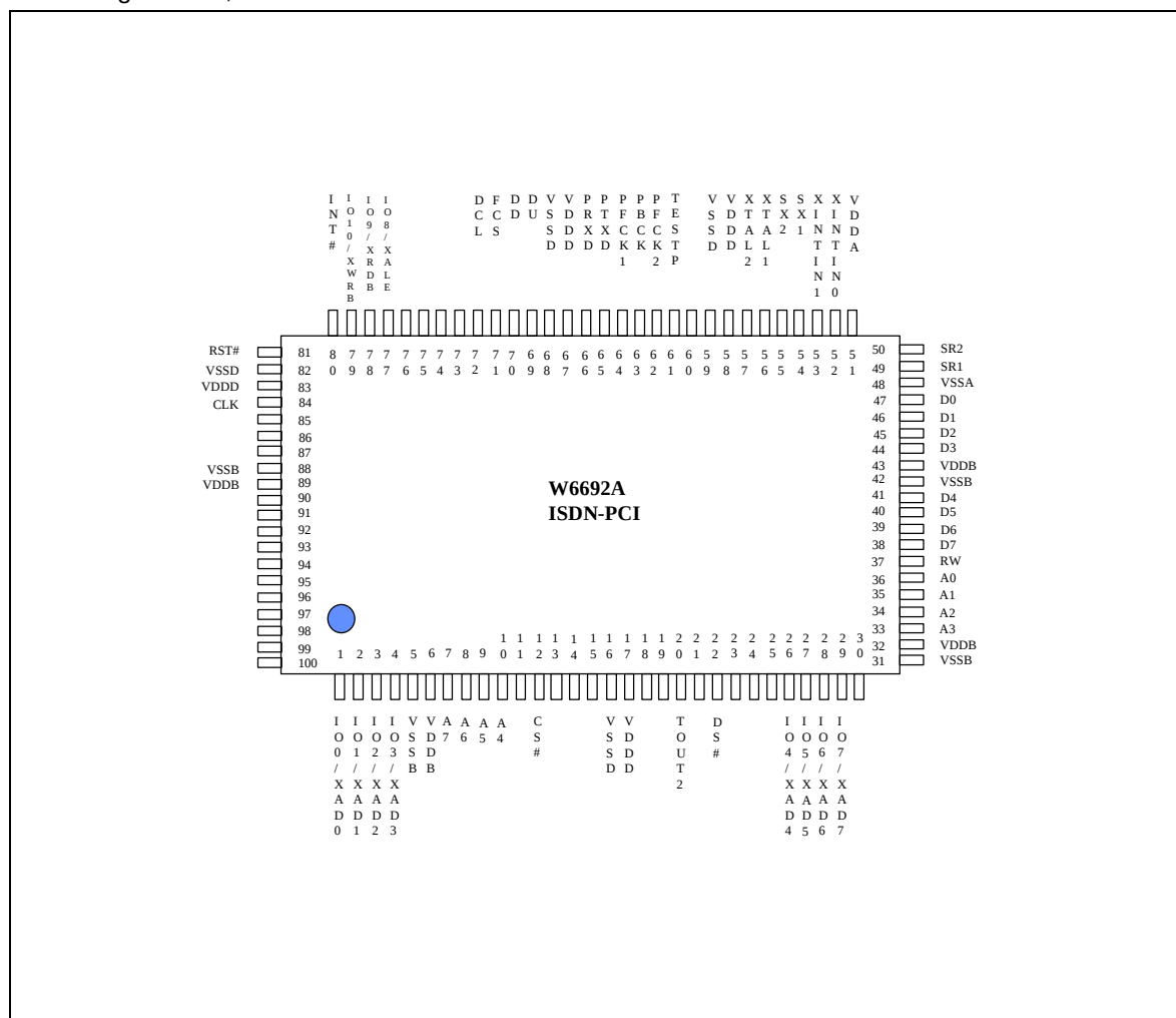
Fig.3.3 W6692A Pin Configuration - Motorola Bus Mode
