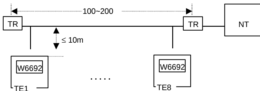
(b) Short passive bus configuration
