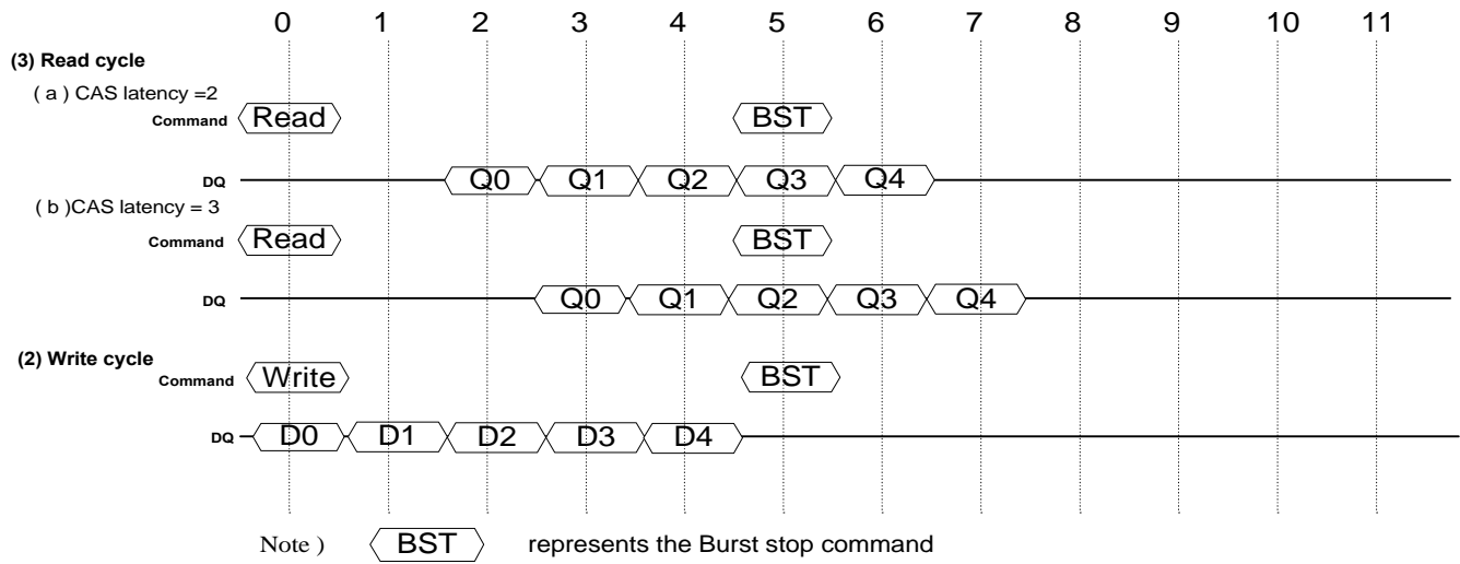
Timing chart of Burst Stop cycle ( Burst stop Command )
