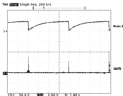
Figure 10. Automatic Restart After Current Fault
